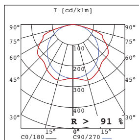
Lichtdiagram UNN249 + RT1/2-B + LRT32
